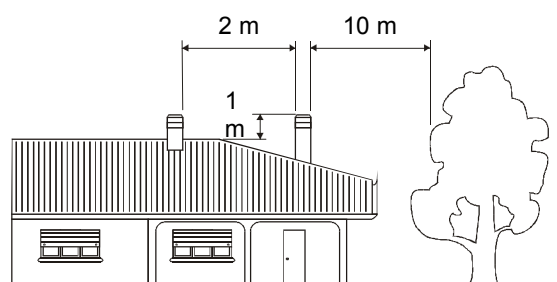
(1) The chimney cap must not show hindrances within 10 m from walls, pitches and trees. Otherwise raise it of at least 1 m over the hindrance. The chimney cap must exceed the ridge of the roof of at least 1 m.
